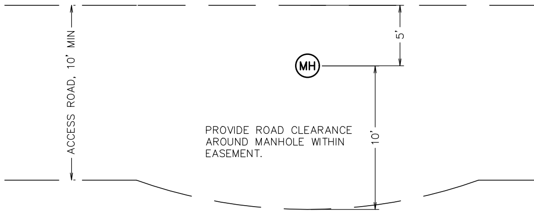
MANHOLES OUTSIDE OF VEHICULAR TRAFFIC AREAS
