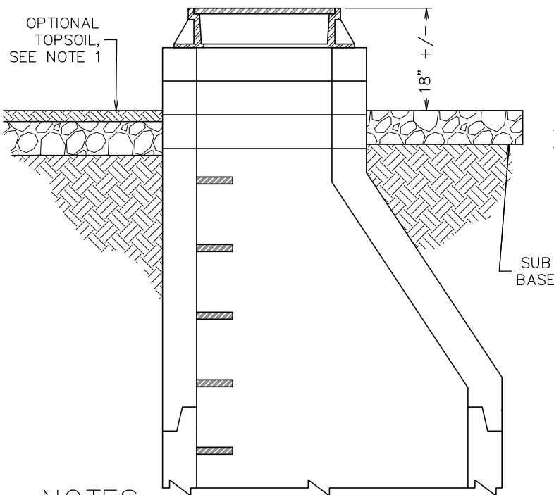
MANHOLES OUTSIDE OF VEHICULAR TRAFFIC AREAS
