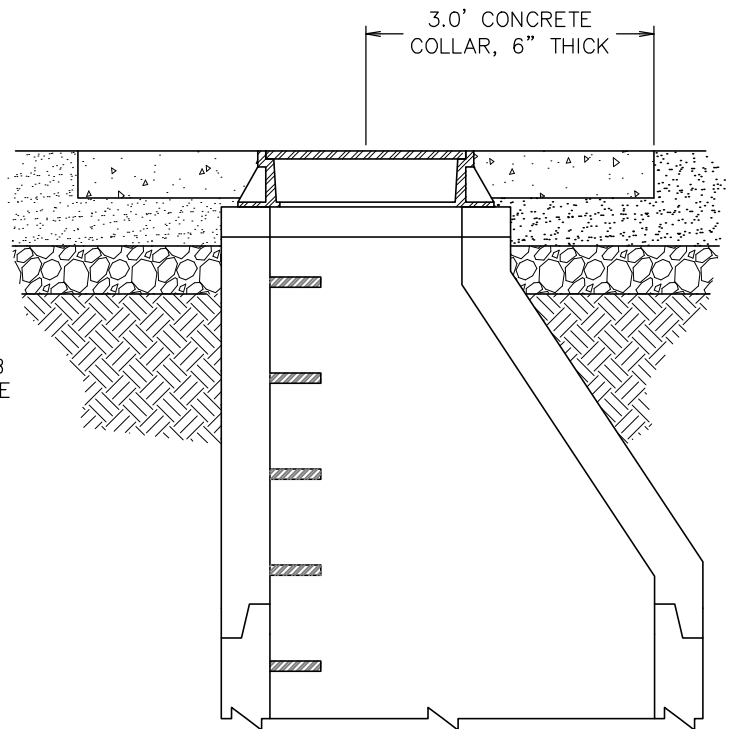
MANHOLES IN VEHICULAR TRAFFIC AREAS
